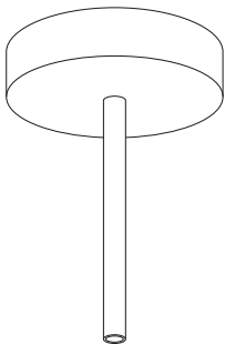
KRM57FCG00TERM5 1 HOLE + 150MM CLAMP 120MM H 25MM
