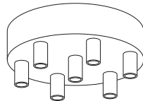
KRM576FBRTERM 7 HOLE Ø 120MM H 25MM
