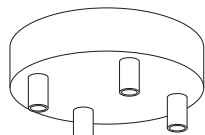
KRM574FRASTERM 4 HOLE Ø 120MM H 25MM
