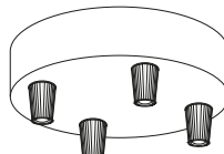
KRM574FV0TS 4 HOLE Ø 120MM H 25MM
