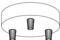
KRM573FVTIS 3 HOLE Ø 120MM H 25MM
