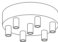
KRM576FRASTERM 7 HOLE Ø 120MM H 25MM
