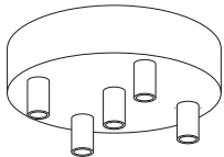
KRM575FG0TERM 5 HOLE Ø 120MM H 25MM
