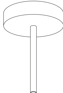
KRM57FCV0TSTERM5 1 HOLE + 150MM CLAMP 120MM H 25MM
