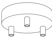
KRM573FVB0TERM 3 HOLE Ø 120MM H 25MM
