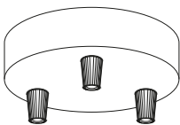
KRM573FVB0 3 HOLE Ø 120MM H 25MM
