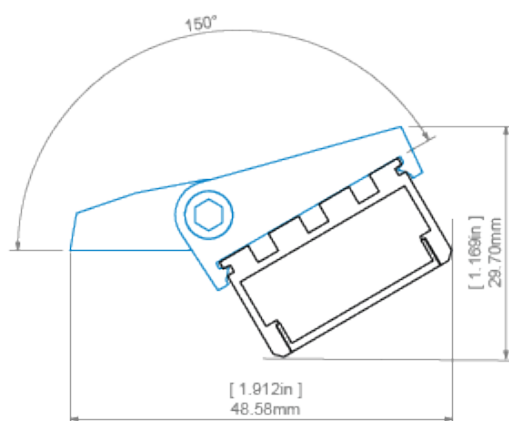
GIZA-LL profile and REGIP-UV mounting bracket profil GIZA-LL z mocowníkem REGIP-UV
