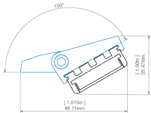
GIZA profile and REGIP-UV mounting bracket profil GIZA z mocowníkem REGIP-UV
